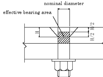
Fig.C11.6.4 Effective bearing area of flat-head bolt
