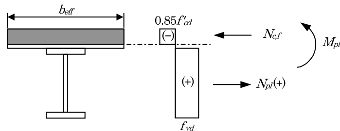
(a) When plastic neutral axis is within the concrete deck in positive bending
