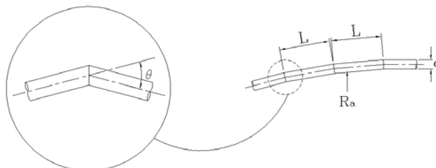
Fig.C10.6.5 Bent tube
