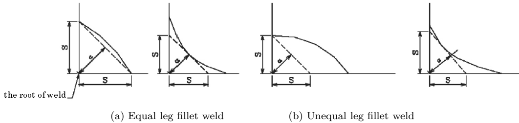
Fig.C11.5.4 Theoretical throat thickness of fillet weld
