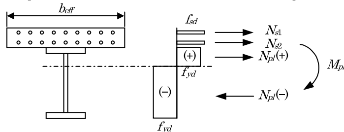
(b) When plastic neutral axis is within the web receiving negative bending
