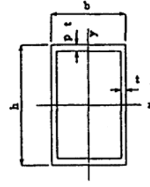
Fig.C5.3.2 Dimension of box-section
