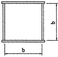
Fig.C5.3.4 Distance between the fixed edges of plate supported at both ends
