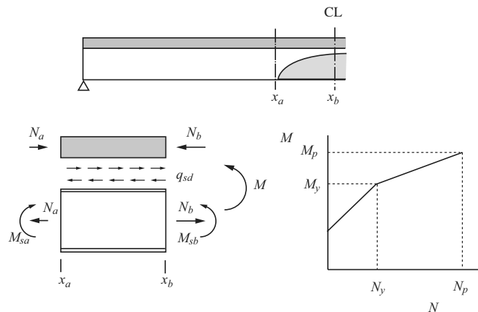
Fig.C15.4.3 Relationship between bending moment and axial force of concrete deck
