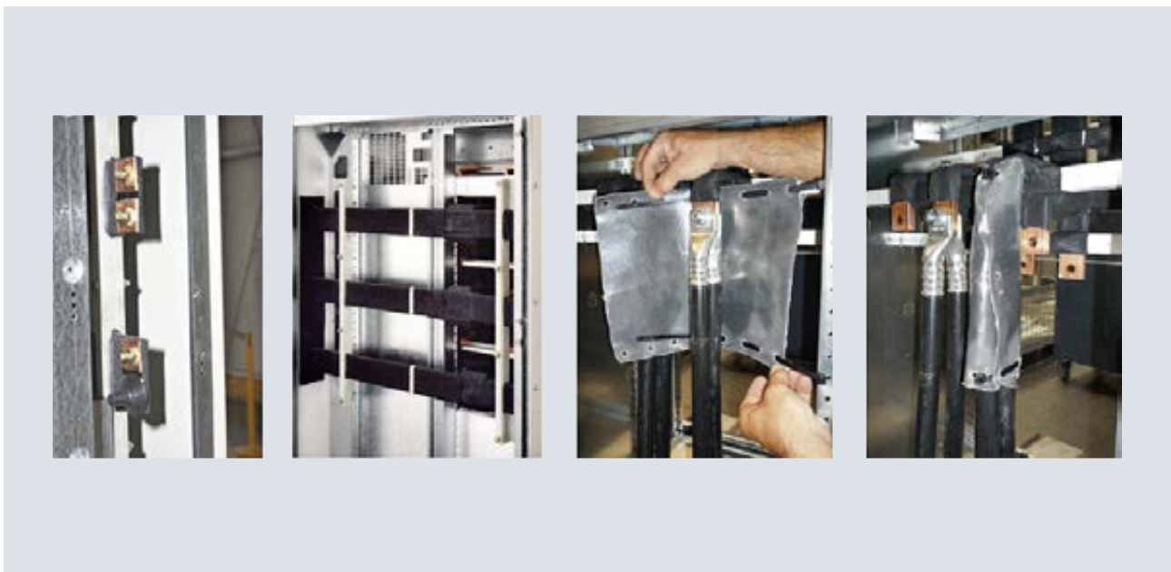
Fig. 10/9: Passive system to prevent arcing faults with insulated busbar, panel connector, incoming and outgoing feeder
