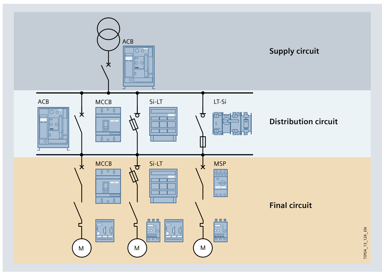
Fig. 11/2: Protection device matrix according to circuit type
