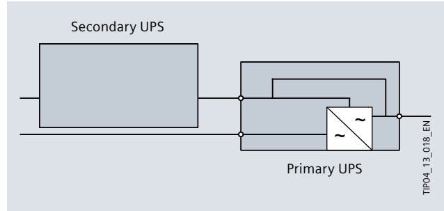
Fig. 5/10: Schematic illustration of the standby redundancy for a single UPS system back to page 82
