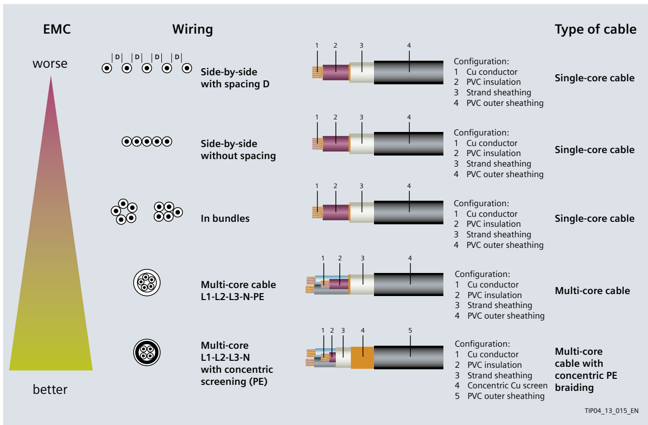
Fig. 5/7: Classification of simple cable types and wiring with regard to EMC
