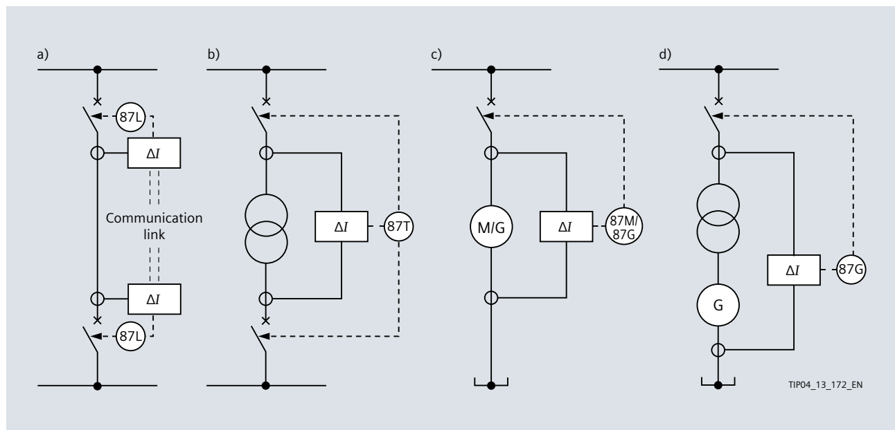
Fig. 8/14: Block diagrams for a) line differential protection b) transformer differential protection ( S_{rT} > 10 MVA) c) motor/generator differential protection ( P_{rM} > 2 MW/ P_{rG} > 1 MW) d) generator blocking protection ( P_{rG} > 1 MW)
