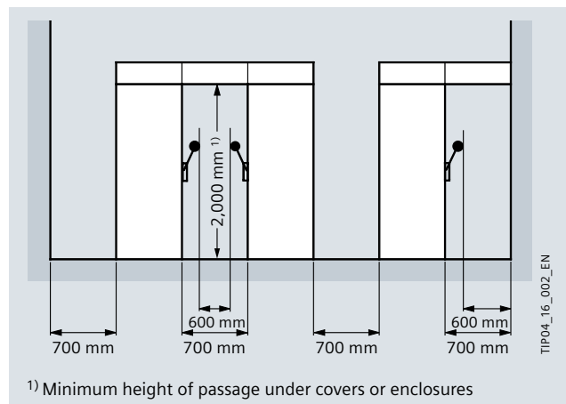
Fig. 10/5: Maintenance gangway widths and passage heights
