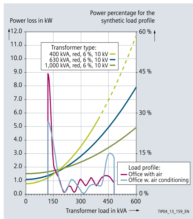
Fig. 14/8: Comparison of the power losses of various GEAFOL transformer types (high voltage 10 kV, red = reduced losses, rated short-circuit voltage u_{zr} = 6\% ) and synthetic load profiles for office building types
