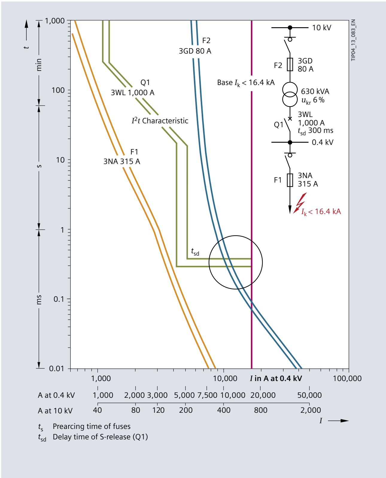
Fig. 7/35: Example of grading a HV HRC fuse F2 with circuit-breaker Q1 and downstream LV HRC fuse F1 in the branch circuit
