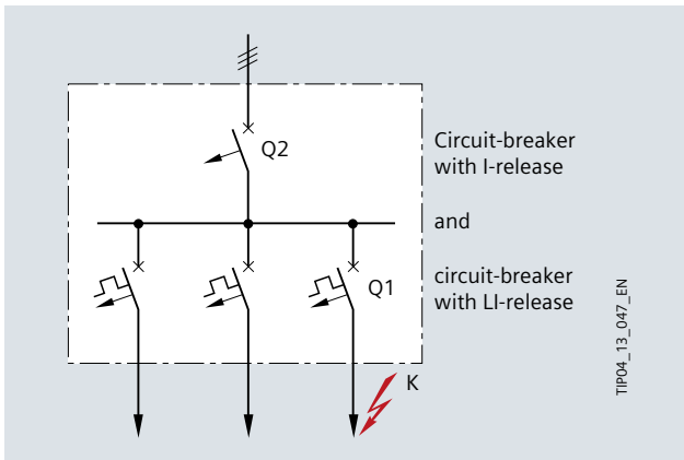
Fig. 7/2: Setting possibilities for Siemens circuit-breakers
