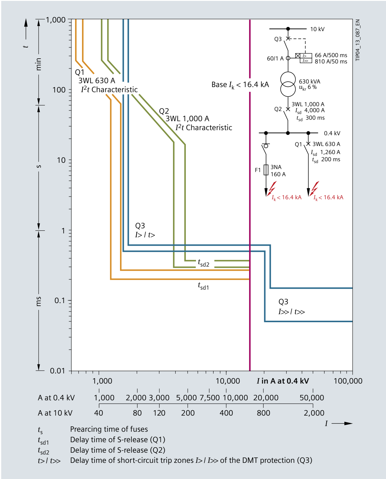
Fig. 7/39: Example of grading a circuit-breaker with DMT protection (Q3), 3WL circuit-breaker, 1,000 A with LSI-release (Q2) and downstream branch circuits with 3WL circuit-breaker, 630 A, LSI-release (Q1), in a transformer branch circuit supplying 630 kVA back to page 150
