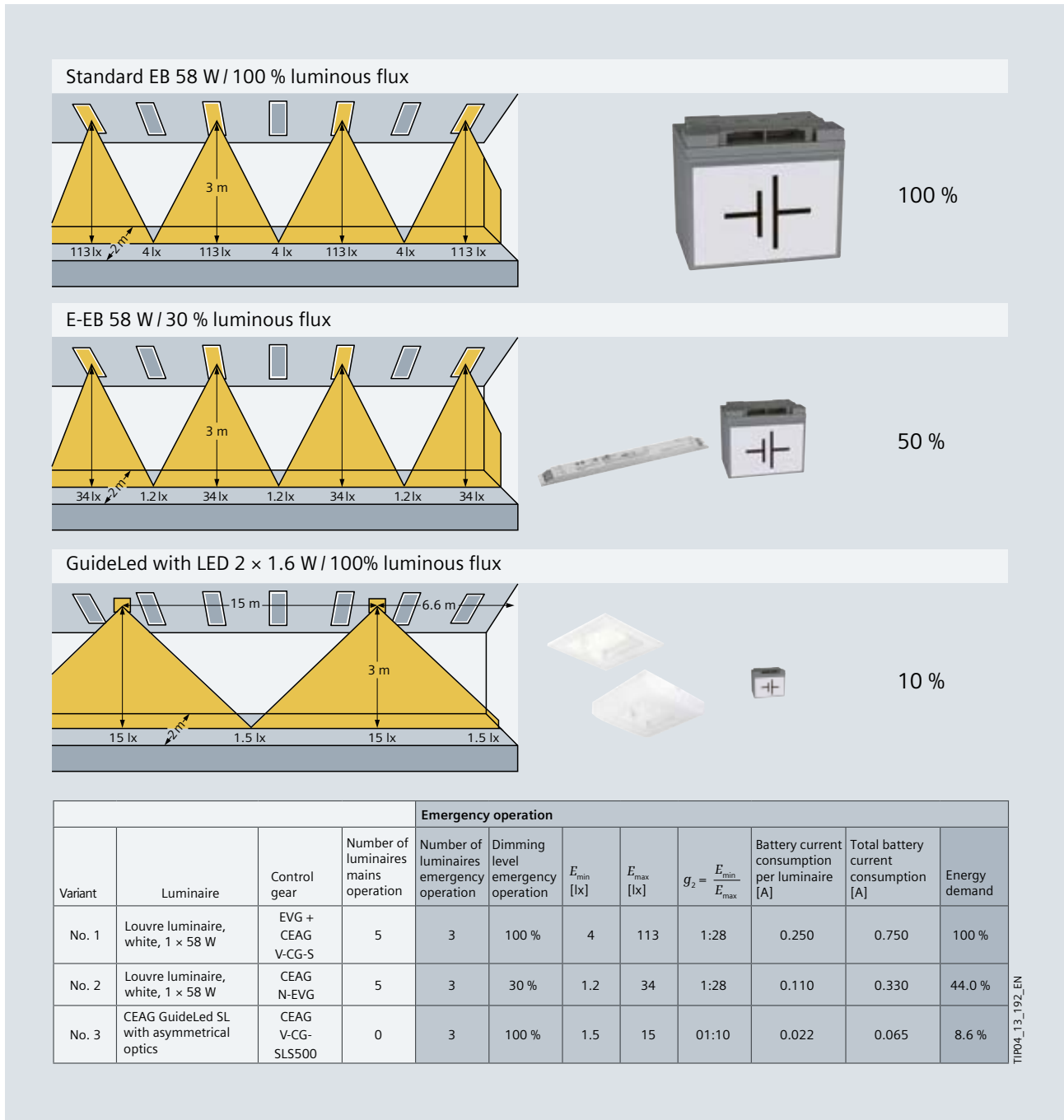
Fig. 16/19: Lighting engineering instead of battery use
