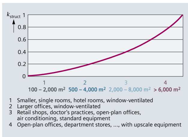
Fig. 2/3: Schematic dependency of the power demand from the building structure demonstrated through a standardised factor k_{struct}
