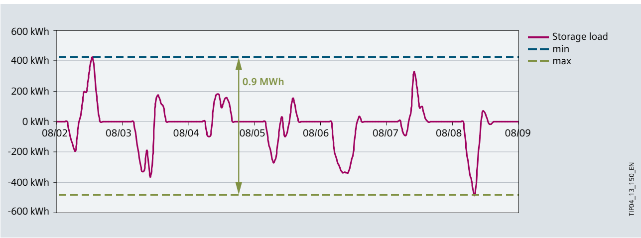
Fig. 13/15: Weekly curve of the energy required which a storage system is to supply, respectively take in, based on the power ratios from Fig. 13/14 back to page 275
