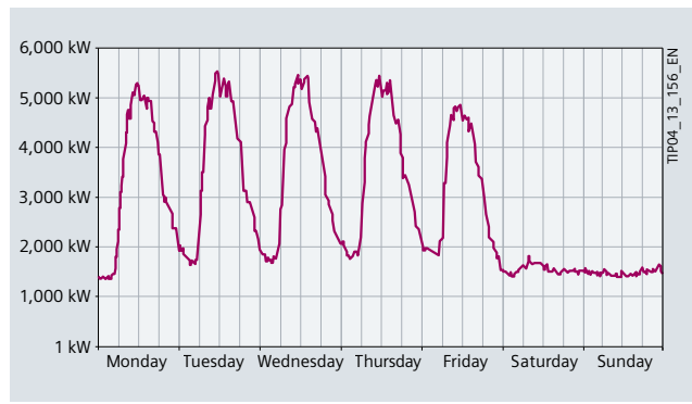
Fig. 14/5: Weekly load curves for a measuring point
