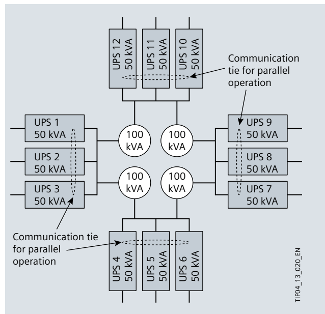
Fig. 5/12: Isolated-parallel UPS system with a link through two independent power supply units acc. to (m+1)^{(n+1)} – here: (3+1)^{(2+1)} back to page 82
