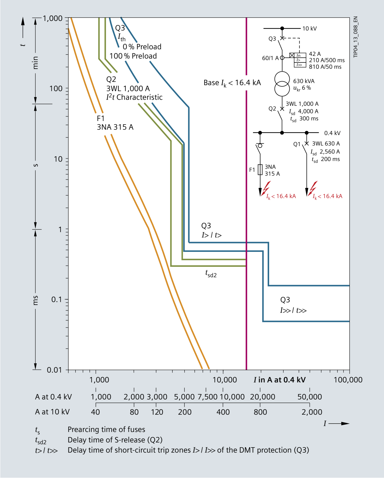
Fig. 7/40: Example of grading a circuit-breaker with DMT protection and overload protection (Q3), 3WL circuit-breaker, 1,000 A with LSI-release (Q2) and downstream branch circuits with LV HRC fuse 315 A (F1), in a transformer branch circuit supplying 630 kVA
