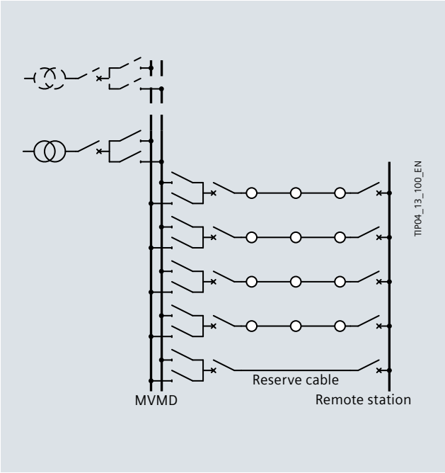
Fig. 4/4: Network configuration: lines with remote station
