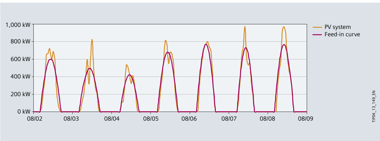
Fig. 13/14: Weekly curve of PV power and the desired feed-in power according to the forecast about sun radiation provided the day before back to page 274
