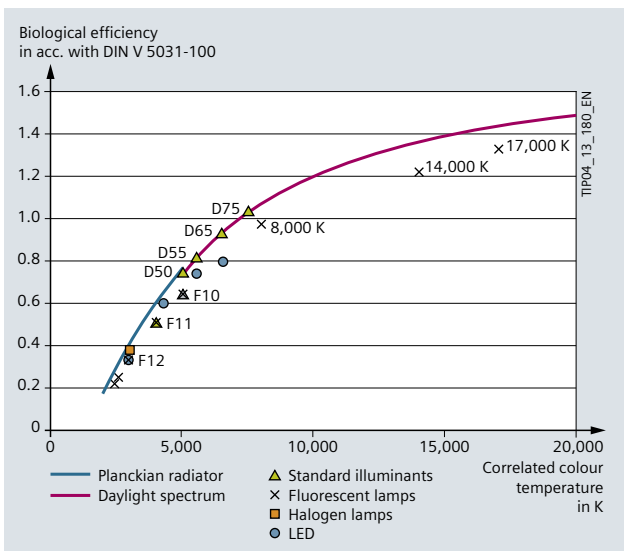
Fig. 16/6: Biological efficiency factors as a function of the correlated colour temperature in accordance with DIN SPEC 67600
