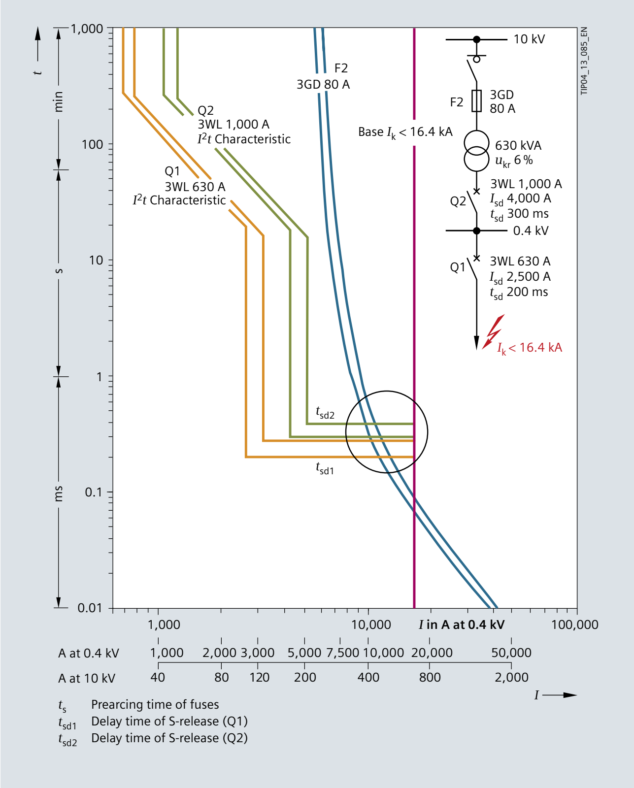
Fig. 7/37: Example of grading a HV HRC fuse F2 with circuit-breaker Q2 and downstream circuit-breaker Q1 with an LSI-release in the branch circuit back to page 149
