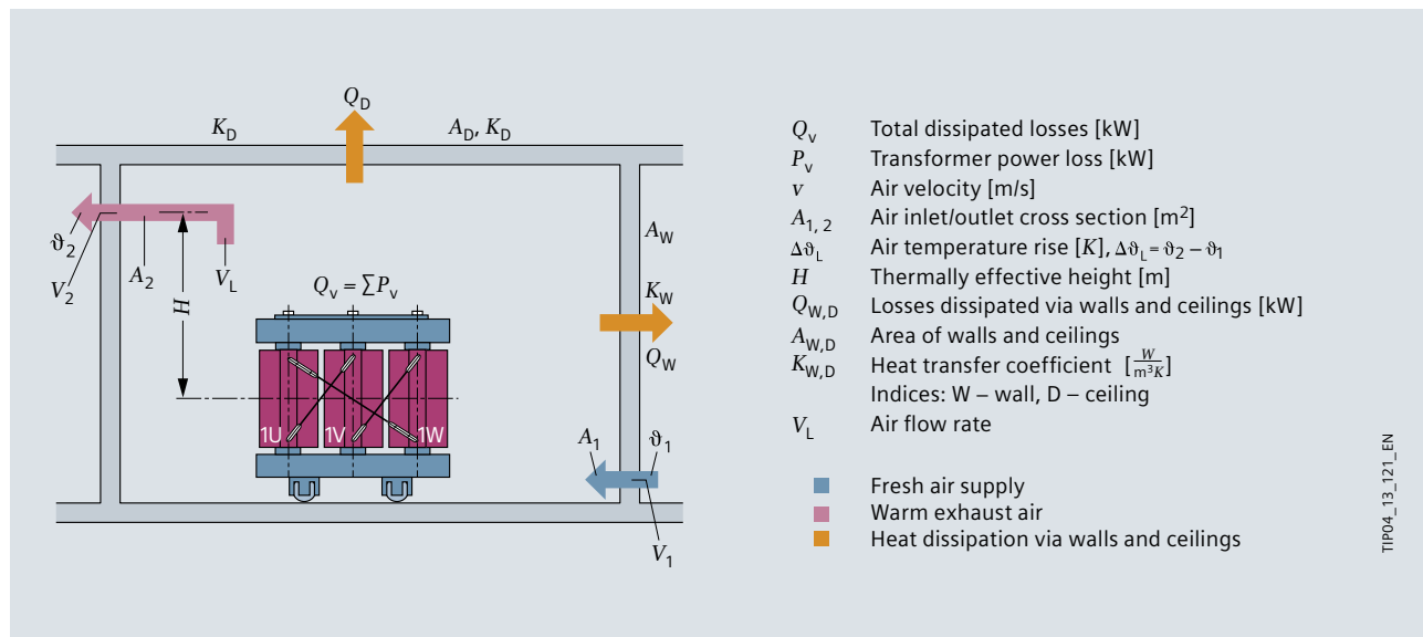
Fig. 9/10: Specifications for the ventilation calculation
