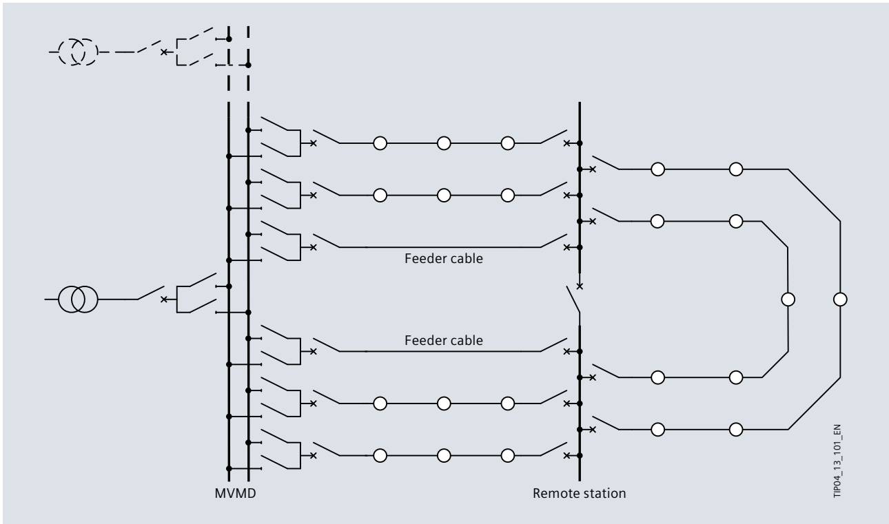
Fig. 4/5: Network configuration: lines with load-centre substation
