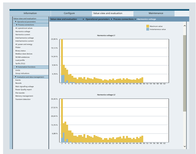
Fig. 5/4: Visualisation of harmonics with SICAM Q100 power quality recorder back to page 73
