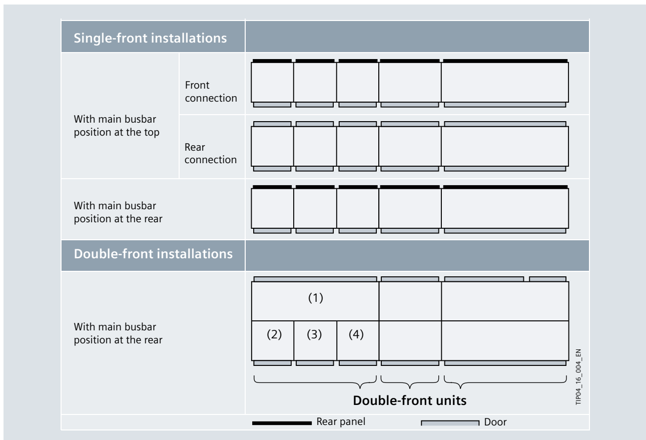
Fig. 10/7: Cubicle arrangement for double-front installations
