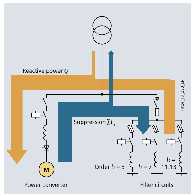
Fig. 5/22: Choked capacitors with thyristor control
