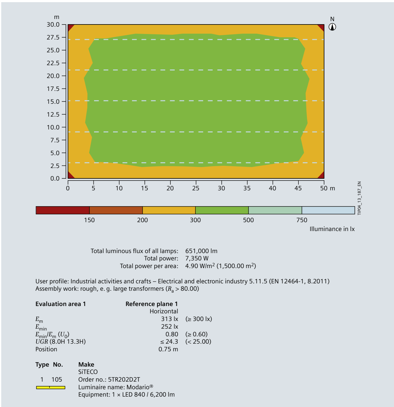
Fig. 16/14: Excerpt of the results of a software calculation for the LED lighting system
