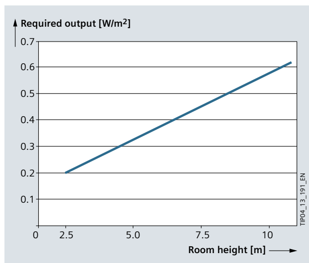
Fig. 16/18: Power estimate for emergency lighting systems with a central battery, based on experience gained with fluorescent lamps at an illuminance of 1 lx back to page 333
