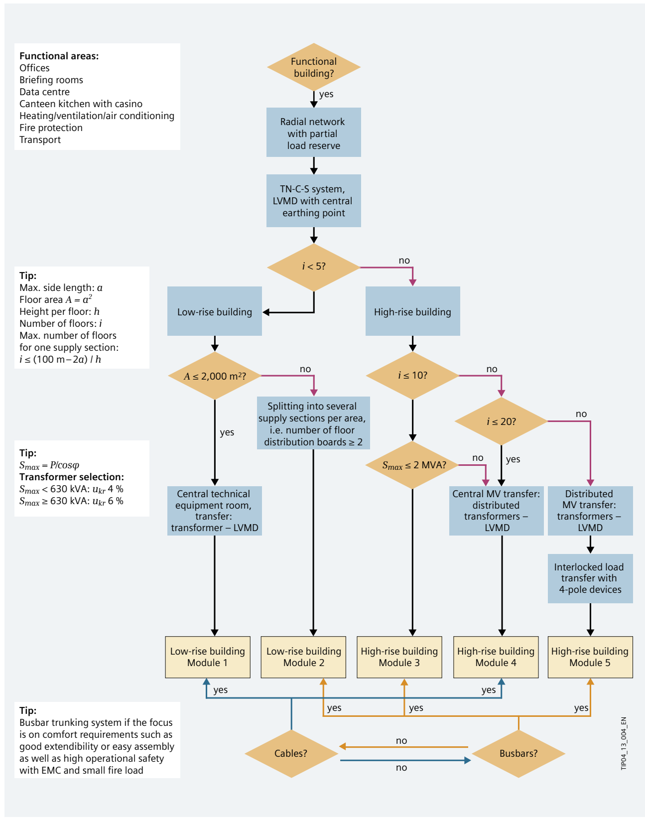
Fig. 3/1: Overview of the network planning concepts
