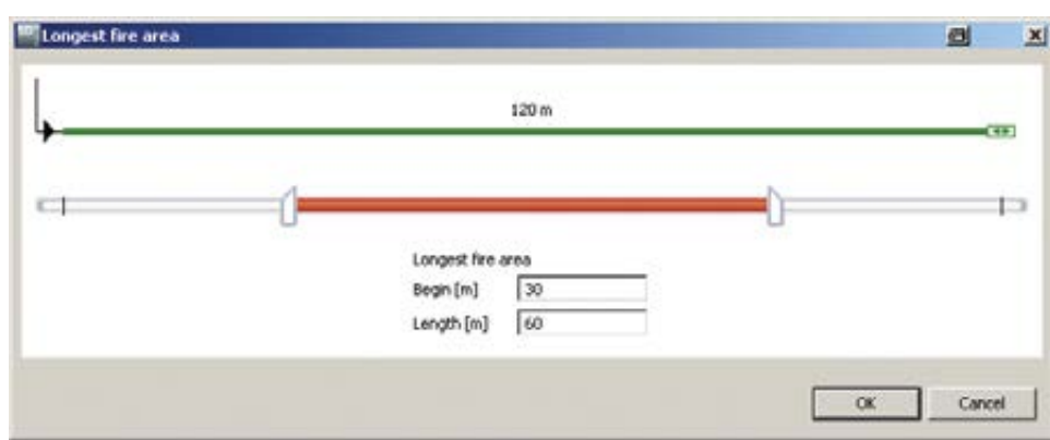
Fig. 15/2: Defining the longest fire section for a busbar trunking system in SIMARIS design
