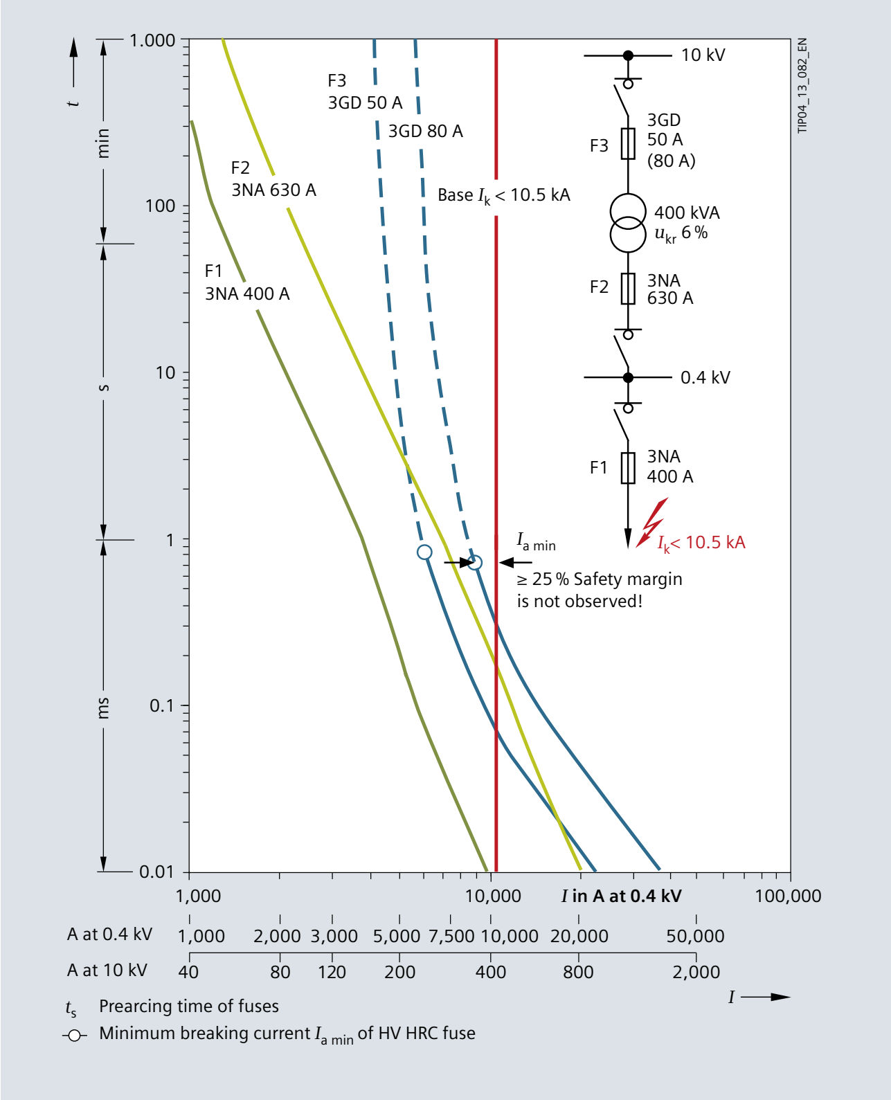
Fig. 7/34: Example of grading HV HRC fuses – LV HRC fuses in the branch circuit and a 400 kVA transformer back to page 149
