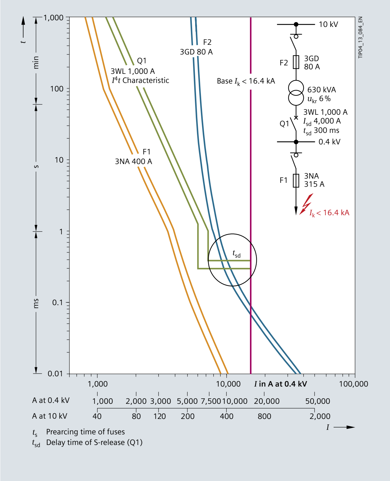
Fig. 7/36: Example of grading a HV HRC fuse F2 with circuit-breaker Q1 (optional I^4t characteristic of the L-release) and downstream LV HRC fuse F1 in the branch circuit back to page 150
