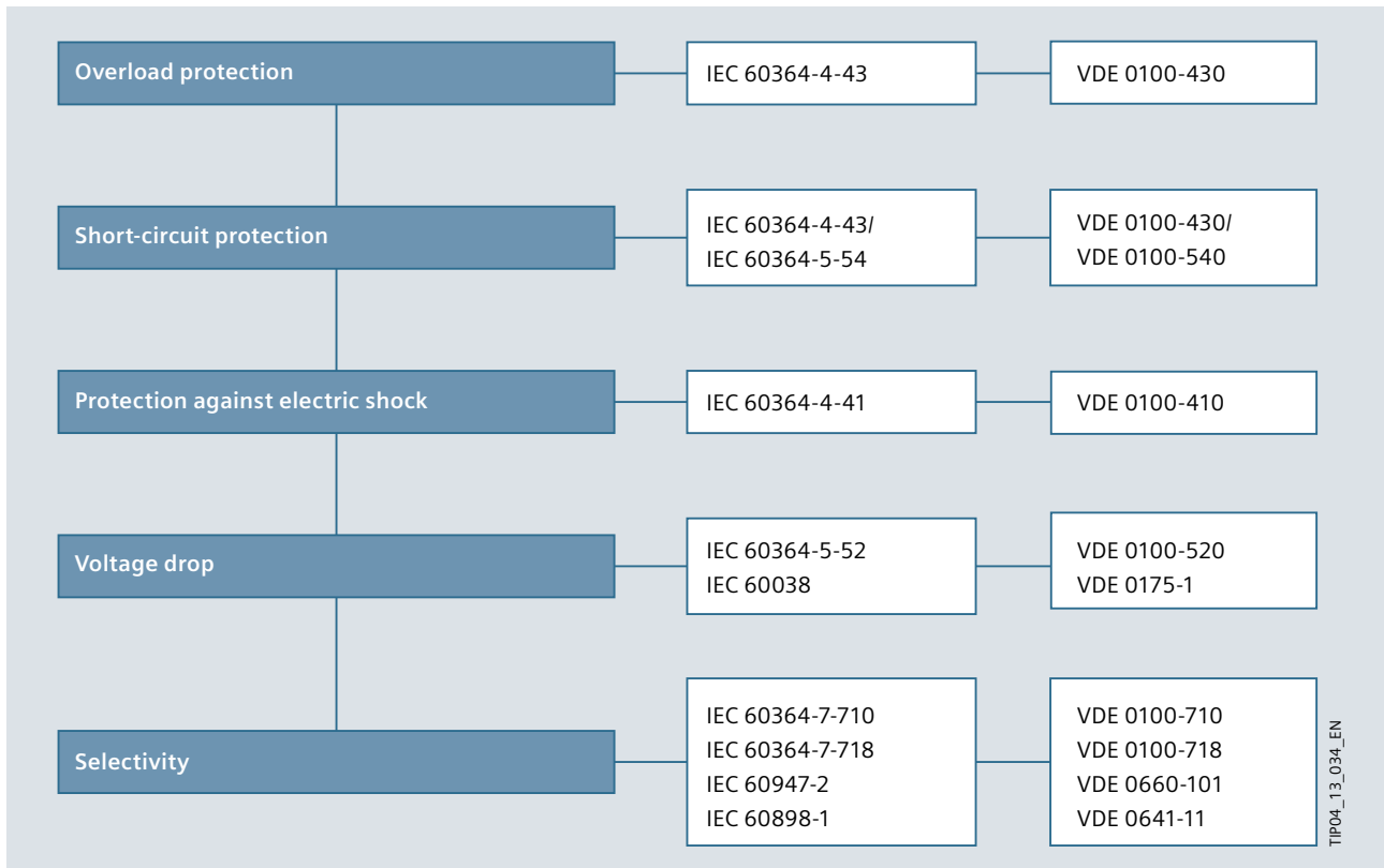
Fig. 6/1: Standards for dimensioning protection devices and routing in circuits
