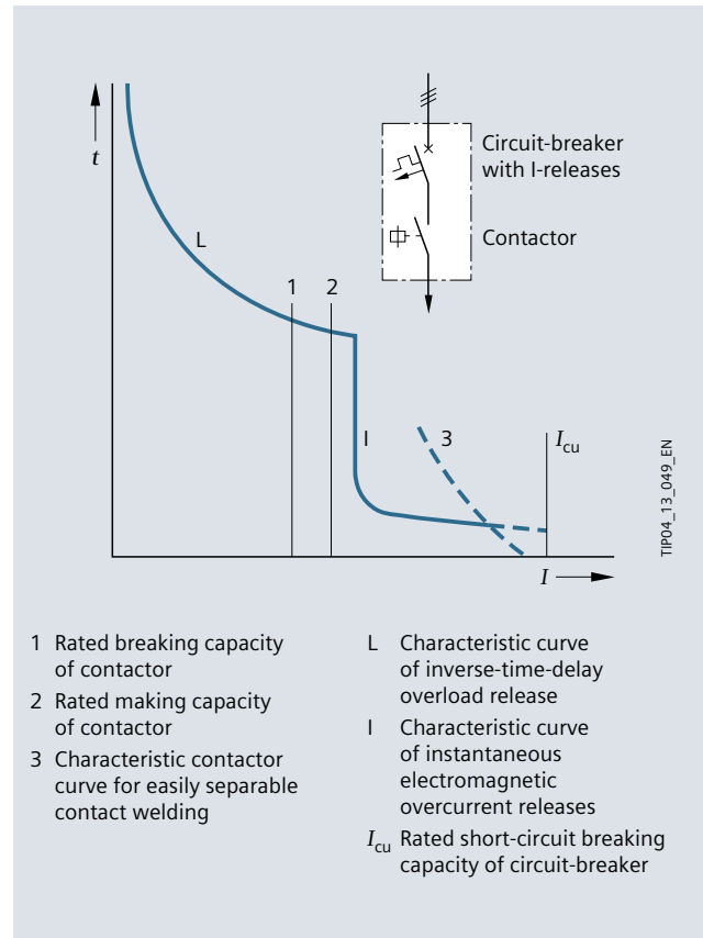
Fig. 7/8: Switchgear assembly comprising circuit-breaker and contactor
