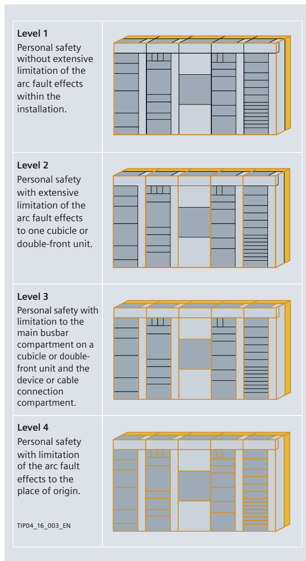
Fig. 10/8: Arc fault levels (installation segments to which the arcing fault is limited are shown orange)
