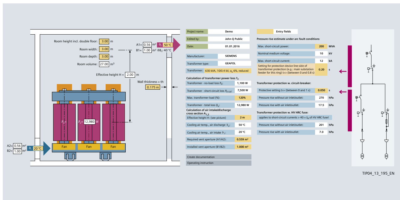
Fig. 9/11: Ventilation of transformer room and approximated pressure rise under arc fault conditions
