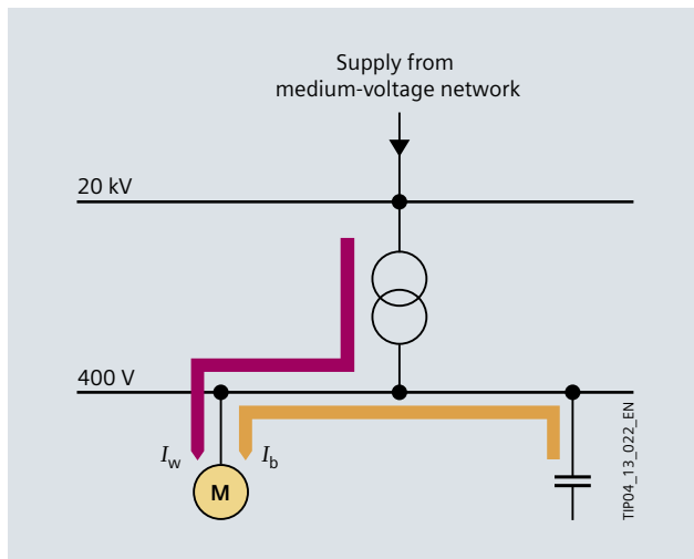
Fig. 5/14: Principle of reactive power compensation using low-voltage power capacitors back to page 84
