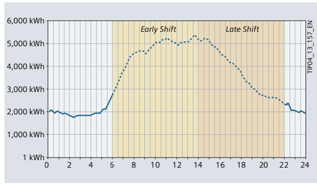
Fig. 14/6: Daily load curve for a measuring point
