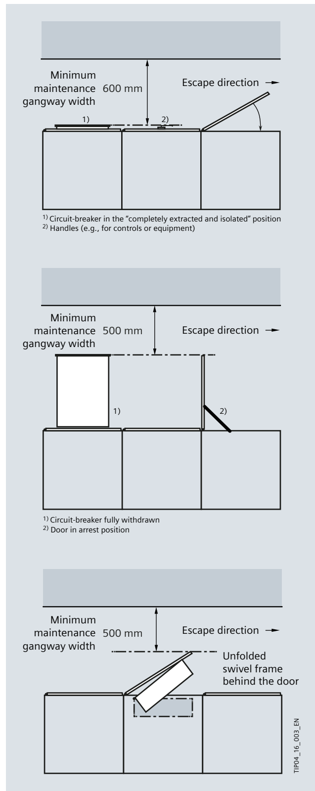
Fig. 10/6: Minimum widths of maintenance gangways in accordance with IEC 60364-7-729 (VDE 0100-729)
