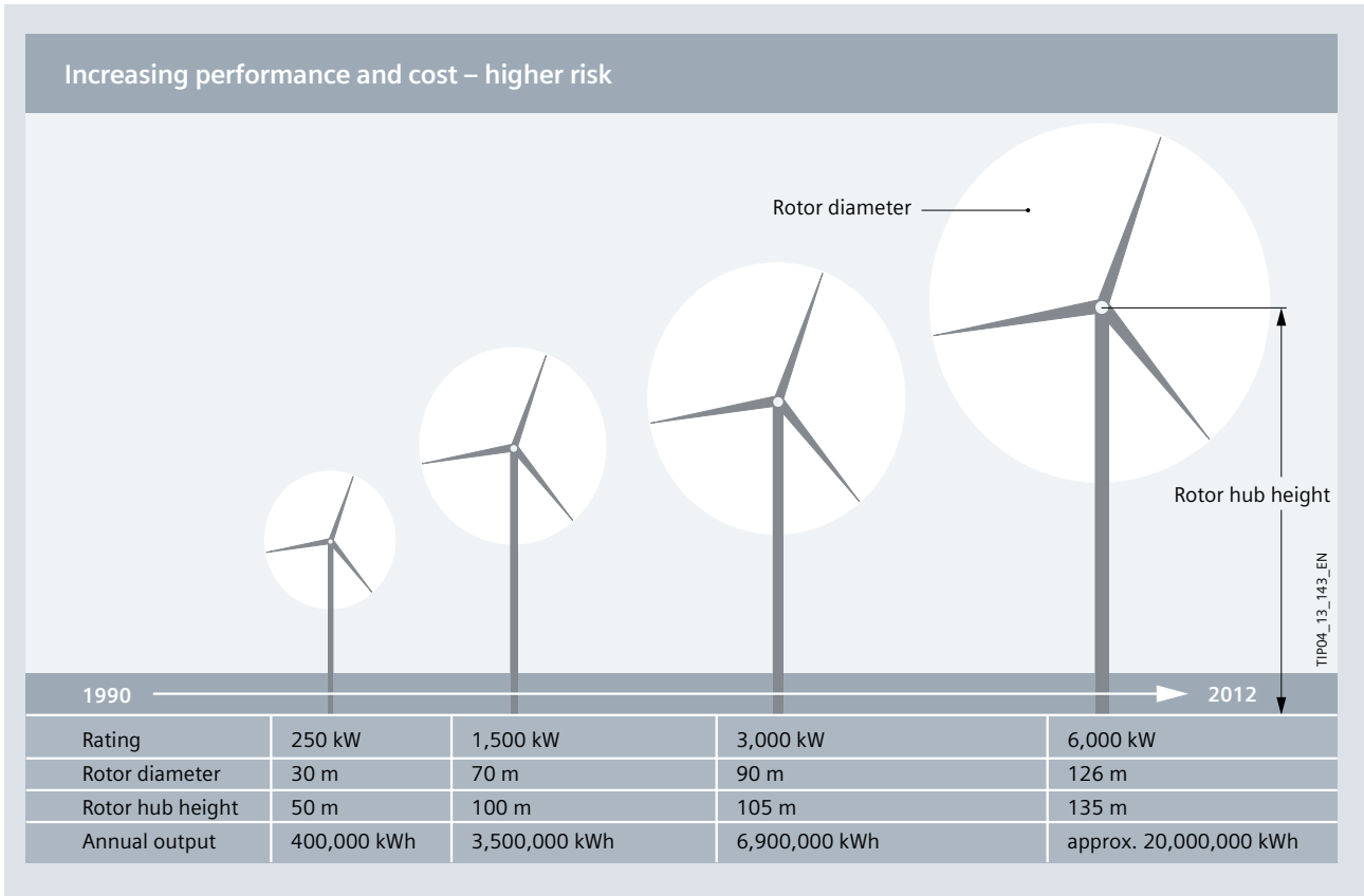
Fig. 13/8: Technical development of wind turbines from 1990 until 2012
