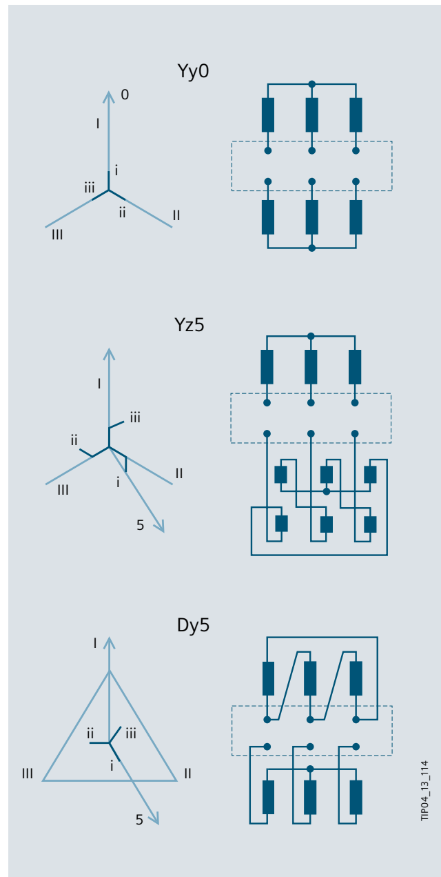
Fig. 9/2: Typical vector groups for three-phase transformers
