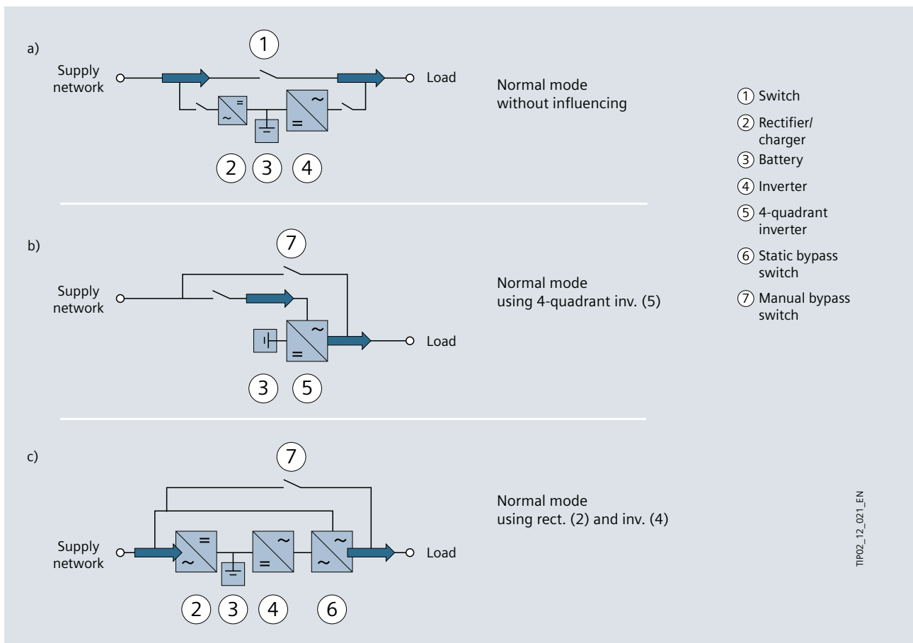
Fig. 13/3: UPS systems with energy flow during normal operation: a) Off-line UPS system (VFD) b) Line-interactive UPS system (VI) c) On-line UPS system (VFI)
