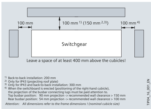
Fig. 10/4: Clearances to obstacles
