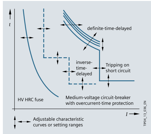
Fig. 6/3: Protection characteristic of HV HRC fuse and MV overcurrent-time protection
