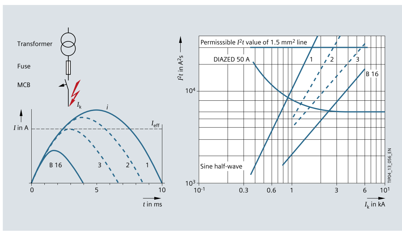
Fig. 7/15: Selectivity of MCBs in current limiting classes 1, 2, and 3 towards back-up fuses (curve B16 applies to Siemens model 16 A, tripping characteristic B) back to page 132
