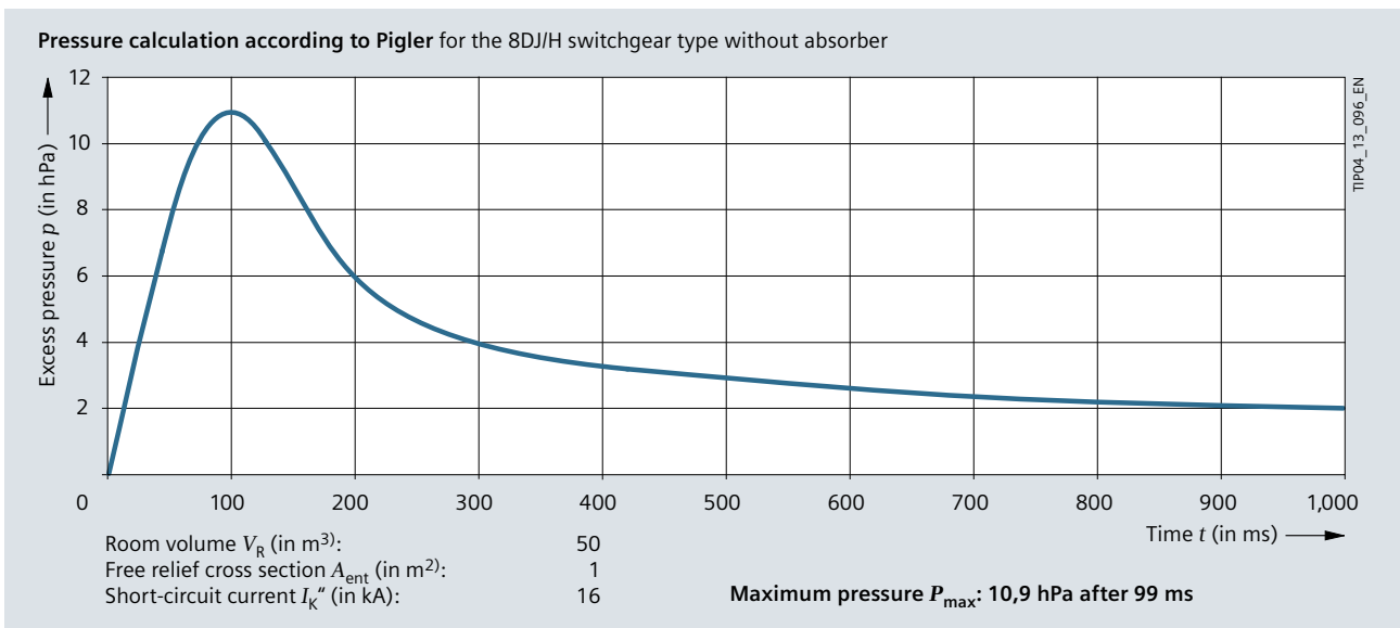
Fig. 8/7: Example of stationary excess pressures resulting from internal arc faults
