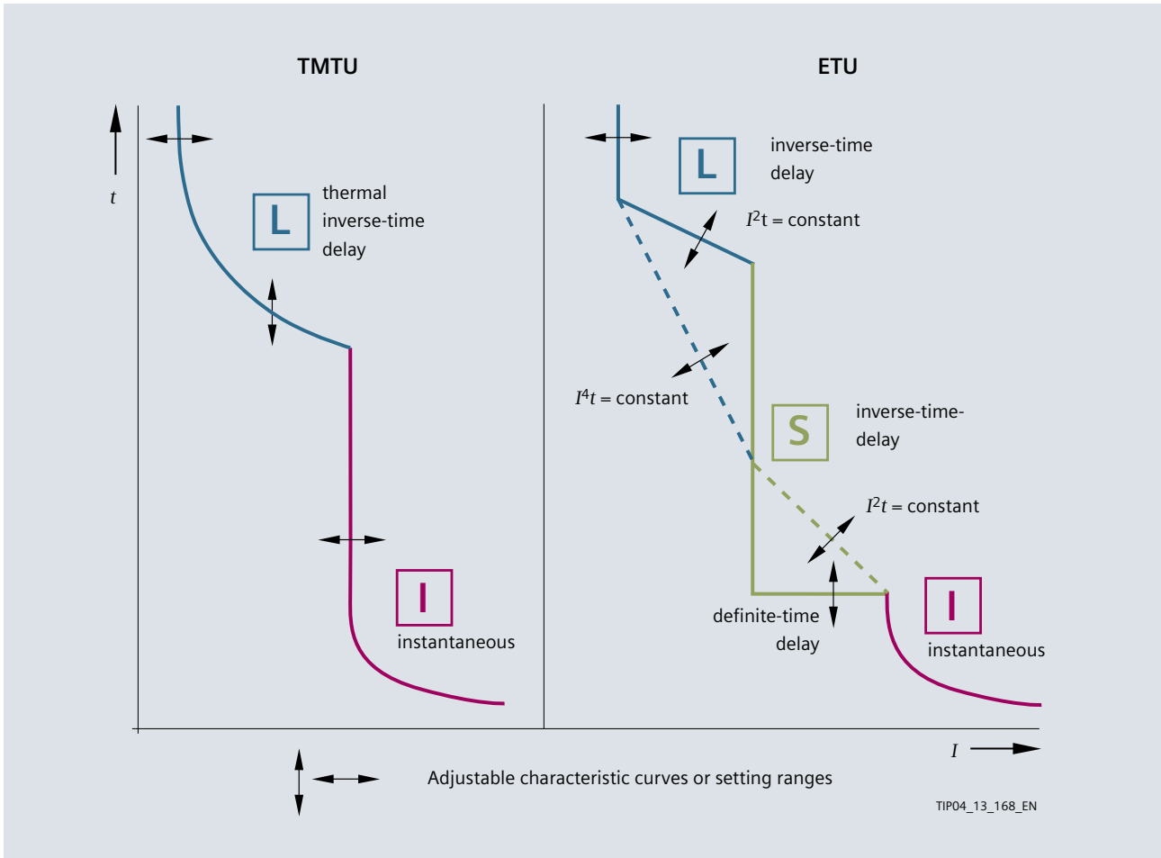
Fig. 7/1: Characteristic tripping curves for low-voltage circuit-breakers
