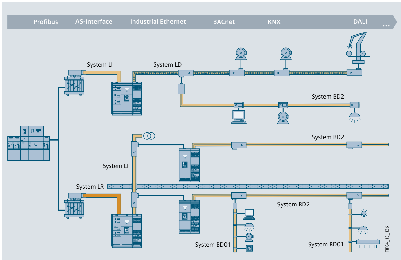
Fig. 10/11: SIVACON 8PS busbar trunking systems for different requirements and loads
