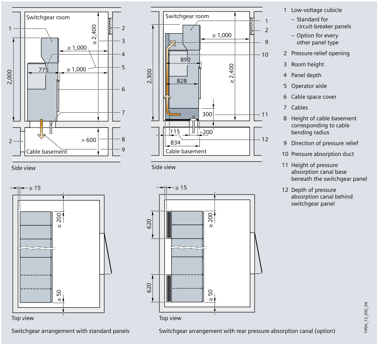
Fig. 8/3: Room layout for switchgear with pressure relief downward (left) and with pressure absorption duct
