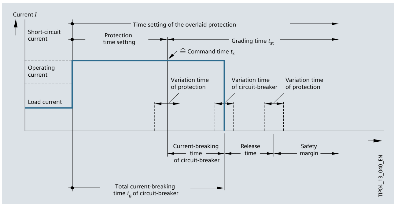
Fig. 6/7: Time grading in medium-voltage switchgear
