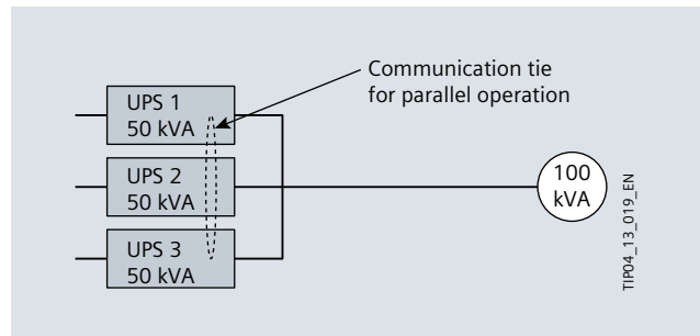
Fig. 5/11: Parallel-redundant UPS system with (n+1) equal to (2+1) back to page 82
