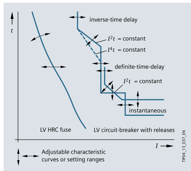
Fig. 6/4: Protection characteristic of LV HRC fuse and LV circuit-breaker with releases
