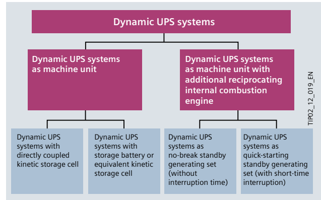
Fig. 13/1: Overview of possible dynamic UPS systems in accordance with DIN 6280-12
