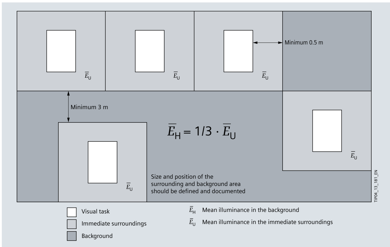
Fig. 16/7: Room structuring for the lighting concept
