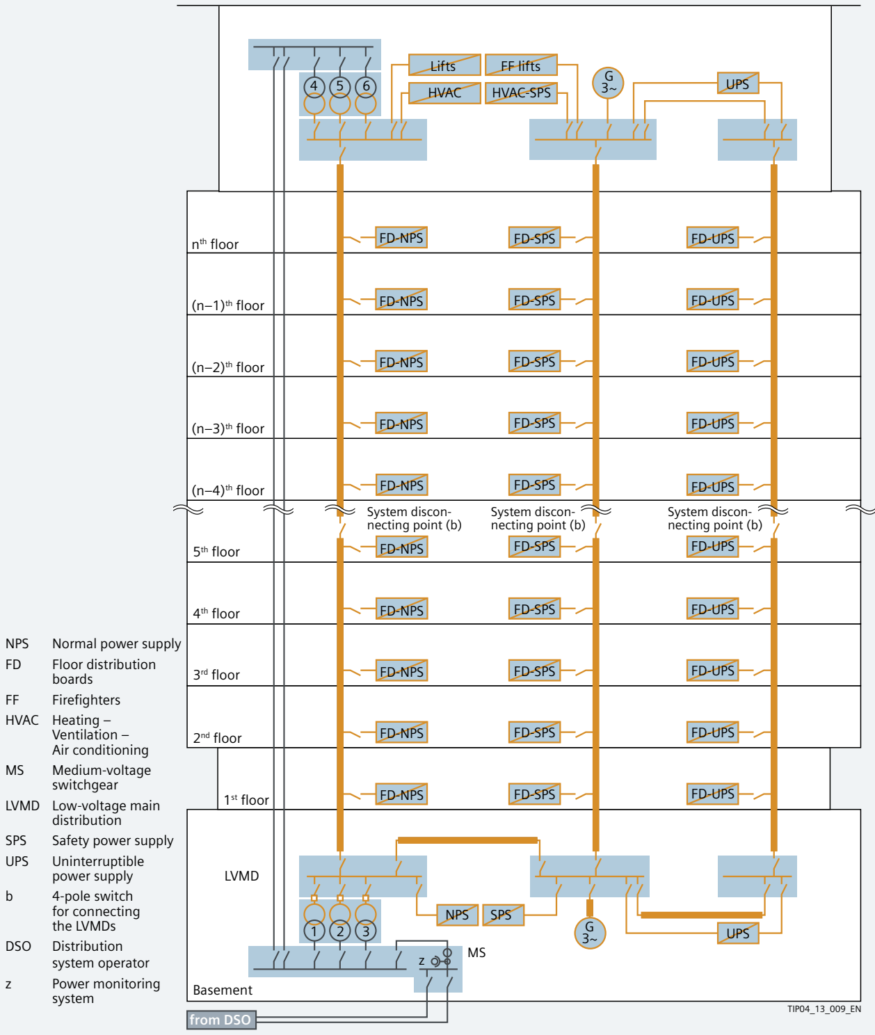
Fig. 3/6: Module 5: High-rise building, busbar, energy center and remote distribution
