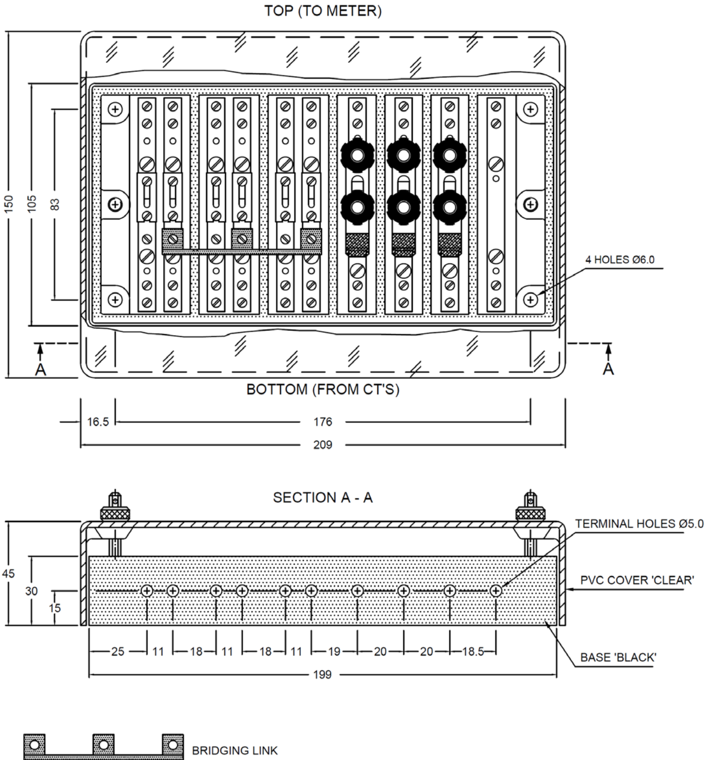
Figure 27 Preferred Test Block Arrangement
