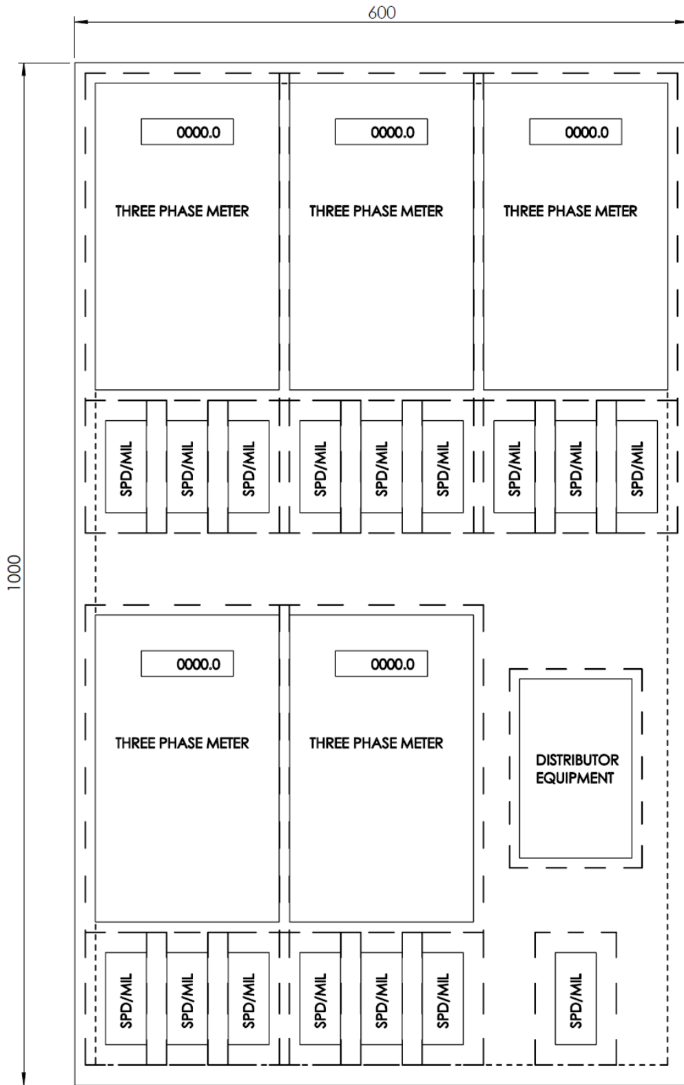
Figure 17 - Typical Panel Layout for Multi Occupancy, multiphase, 1000 x 600 panel
