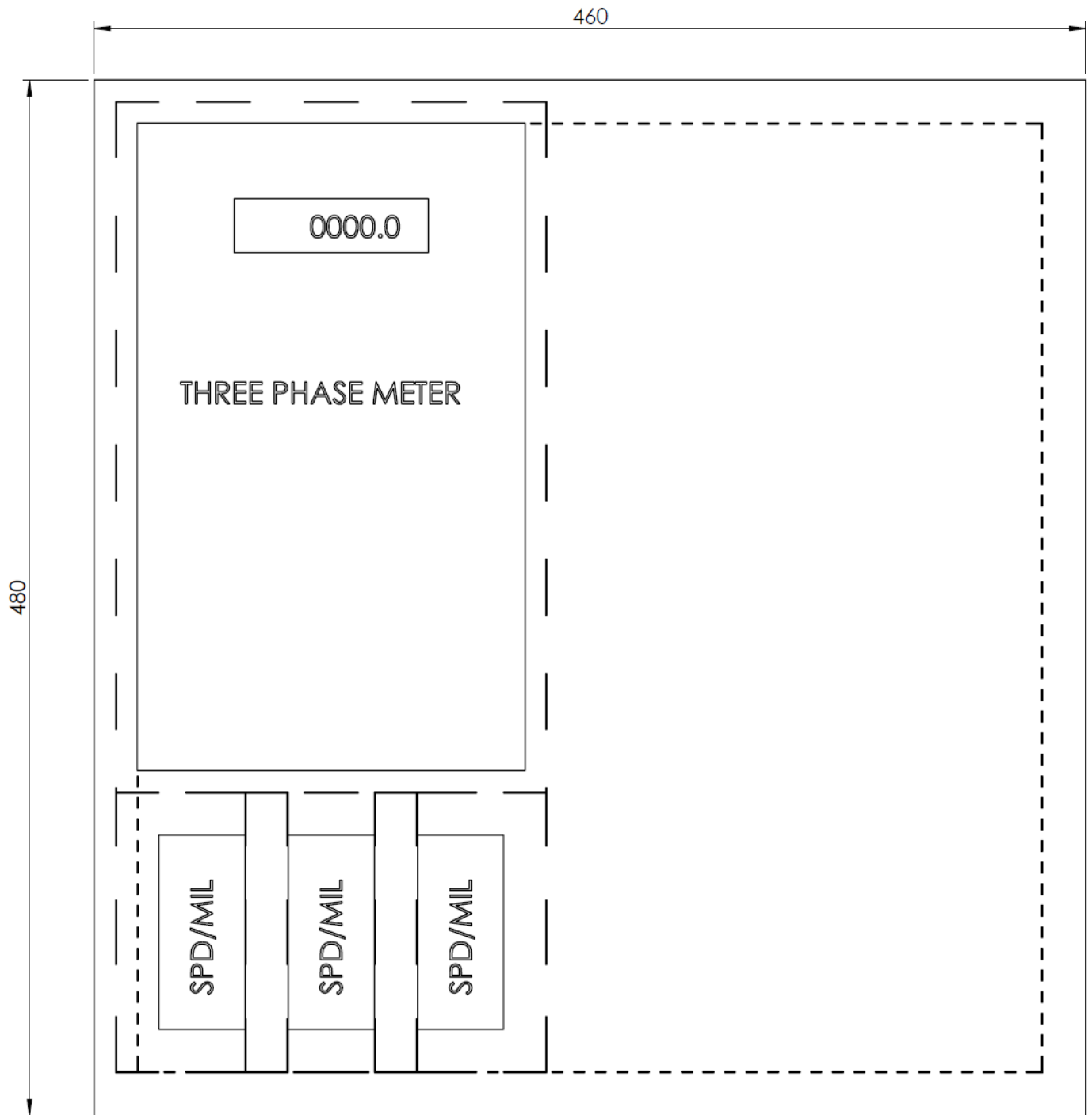
Figure 12 - Typical Panel Layout for Residential House with Multi-phase meter
