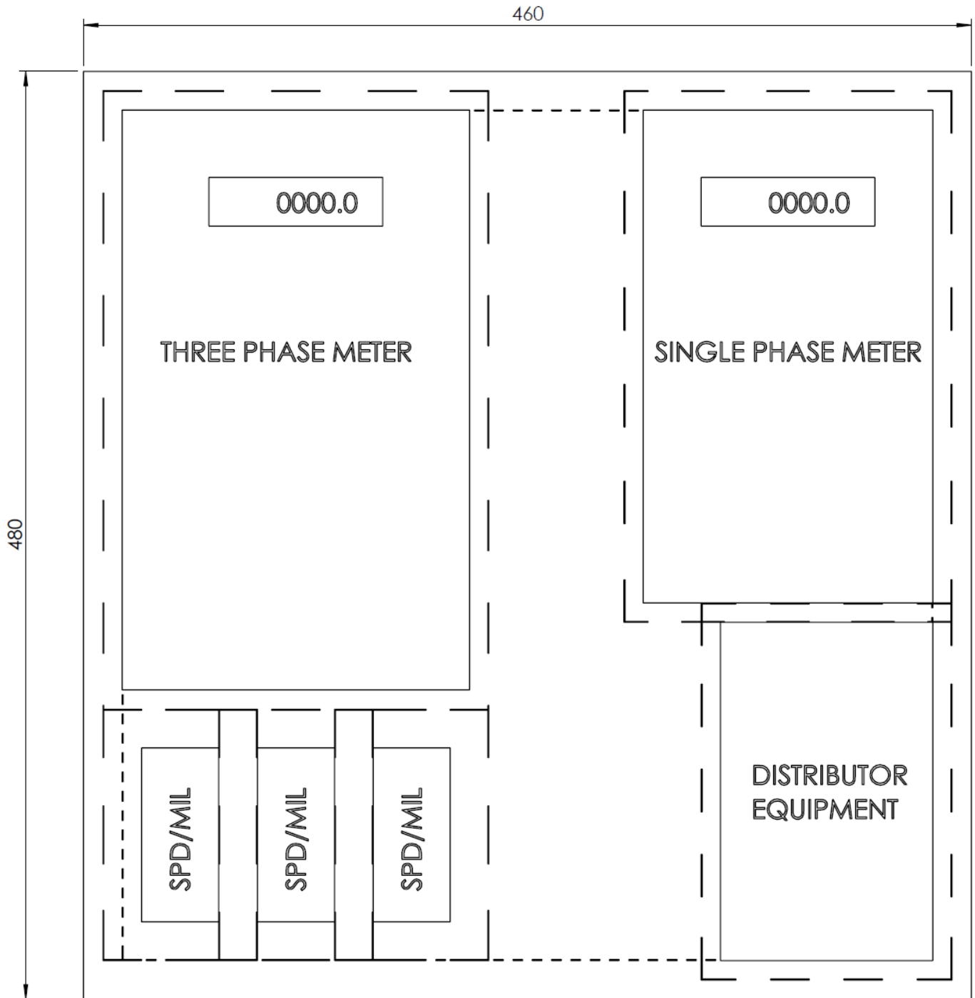
Figure 11 - Typical Panel Layout for Residential House with Multi-phase, single phase meters and load control
