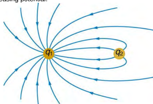
Figure 19.28 The electric field near two charges.
