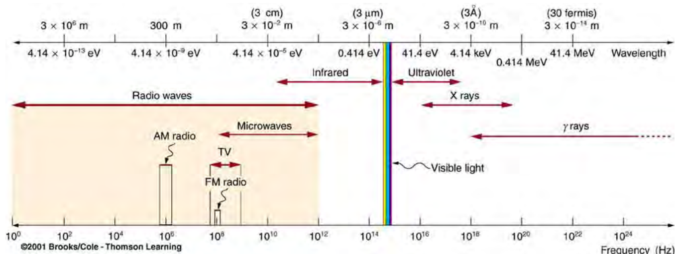
Figure 29.11 The EM spectrum, showing major categories as a function of photon energy in eV, as well as wavelength and frequency. Certain characteristics of EM radiation are directly attributable to photon energy alone.
