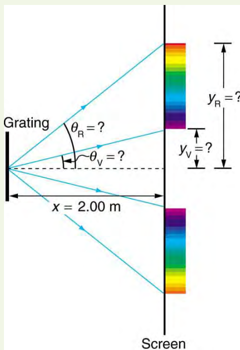
Figure 27.20 The diffraction grating considered in this example produces a rainbow of colors on a screen a distance x = 2.00 m from the grating. The distances along the screen are measured perpendicular to the x -direction. In other words, the rainbow pattern extends out of the page.
