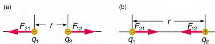
Figure 18.19 The magnitude of the electrostatic force F between point charges q_1 and q_2 separated by a distance r is given by Coulomb's law. Note that Newton's third law (every force exerted creates an equal and opposite force) applies as usual—the force on q_1 is equal in magnitude and opposite in direction to the force it exerts on q_2 . (a) Like charges. (b) Unlike charges.
