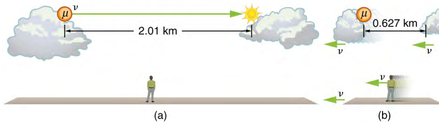
Figure 28.10 (a) The Earth-bound observer sees the muon travel 2.01 km between clouds. (b) The muon sees itself travel the same path, but only a distance of 0.627 km. The Earth, air, and clouds are moving relative to the muon in its frame, and all appear to have smaller lengths along the direction of travel.
