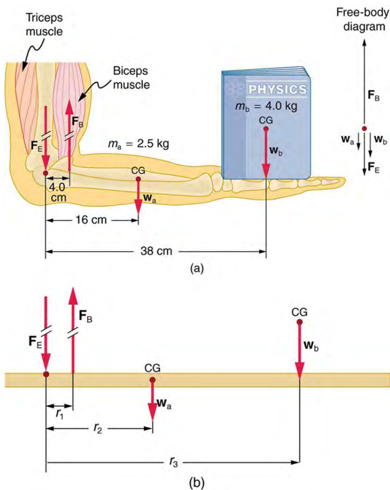
Figure 9.27 (a) The figure shows the forearm of a person holding a book. The biceps exert a force F_B to support the weight of the forearm and the book. The triceps are assumed to be relaxed. (b) Here, you can view an approximately equivalent mechanical system with the pivot at the elbow joint as seen in Example 9.4 .
