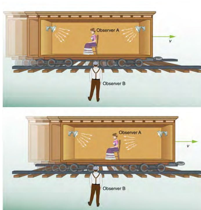
Figure 28.5 Observer B measures the elapsed time between the arrival of light flashes as described in the text. Observer A moves with the lamps on a rail car. Observer B receives the light flashes simultaneously, but he notes that observer A receives the flash from the right first. B observes the flashes to be simultaneous to him but not to A. Simultaneity is not absolute.
