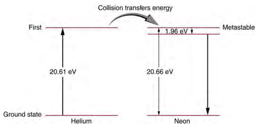
Figure 30.39 Energy levels in helium and neon. In the common helium-neon laser, an electrical discharge pumps energy into the metastable states of both atoms. The gas mixture has about ten times more helium atoms than neon atoms. Excited helium atoms easily de-excite by transferring energy to neon in a collision. A population inversion in neon is achieved, allowing lasing by the neon to occur.
