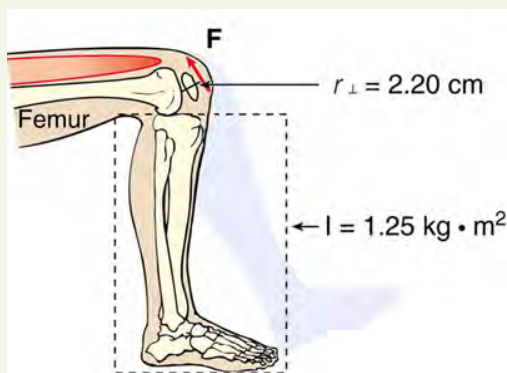
Figure 10.22 The muscle in the upper leg gives the lower leg an angular acceleration and imparts rotational kinetic energy to it by exerting a torque about the knee. F is a vector that is perpendicular to r . This example examines the situation.
