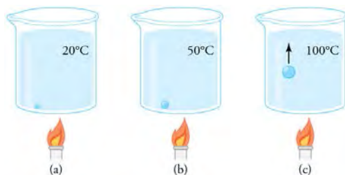
Figure 13.34 (a) An air bubble in water starts out saturated with water vapor at 20^\circ\text{C} . (b) As the temperature rises, water vapor enters the bubble because its vapor pressure increases. The bubble expands to keep its pressure at 1.00 atm. (c) At 100^\circ\text{C} , water vapor enters the bubble continuously because water's vapor pressure exceeds its partial pressure in the bubble, which must be less than 1.00 atm. The bubble grows and rises to the surface.
