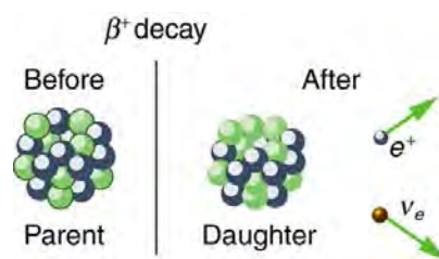
Figure 31.20 \beta^+ decay is the emission of a positron that eventually finds an electron to annihilate, characteristically producing gammas in opposite directions.
