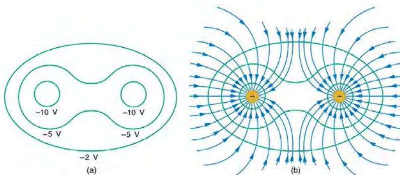
Figure 19.10 (a) These equipotential lines might be measured with a voltmeter in a laboratory experiment. (b) The corresponding electric field lines are found by drawing them perpendicular to the equipotentials. Note that these fields are consistent with two equal negative charges.
