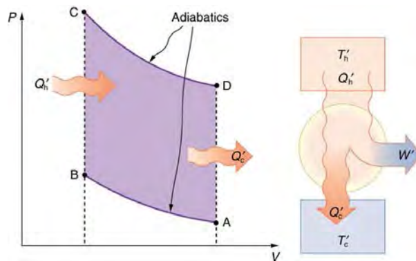
Figure 15.20 This Otto cycle produces a greater work output than the one in Figure 15.19, because the starting temperature of path CD is higher and the starting temperature of path AB is lower. The area inside the loop is greater, corresponding to greater net work output.
