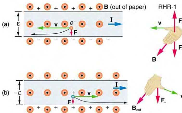
Figure 22.27 The Hall effect. (a) Electrons move to the left in this flat conductor (conventional current to the right). The magnetic field is directly out of the page, represented by circled dots; it exerts a force on the moving charges, causing a voltage \mathcal{E} , the Hall emf, across the conductor. (b) Positive charges moving to the right (conventional current also to the right) are moved to the side, producing a Hall emf of the opposite sign, -\mathcal{E} . Thus, if the direction of the field and current are known, the sign of the charge carriers can be determined from the Hall effect.
