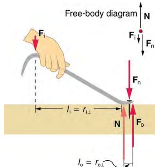
Figure 9.23 A nail puller is a lever with a large mechanical advantage. The external forces on the nail puller are represented by solid arrows. The force that the nail puller applies to the nail ( \mathbf{F}_o ) is not a force on the nail puller. The reaction force the nail exerts back on the puller ( \mathbf{F}_n ) is an external force and is equal and opposite to \mathbf{F}_o . The perpendicular lever arms of the input and output forces are l_i and l_o .
