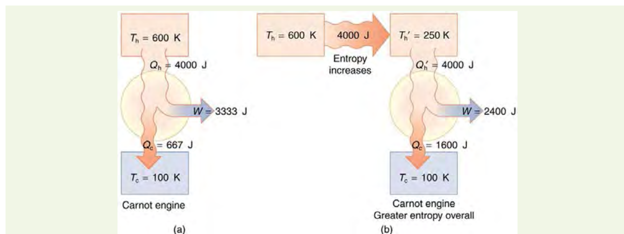
Figure 15.35 (a) A Carnot engine working at between 600 K and 100 K has 4000 J of heat transfer and performs 3333 J of work. (b) The 4000 J of heat transfer occurs first irreversibly to a 250 K reservoir and then goes into a Carnot engine. The increase in entropy caused by the heat transfer to a colder reservoir results in a smaller work output of 2400 J. There is a permanent loss of 933 J of energy for the purpose of doing work.
